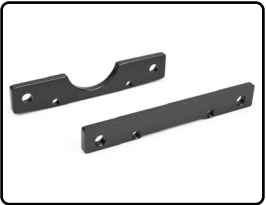
C-00180-418 Suspension Arm Mount - Rear - Aluminum 7075 - 1 set
