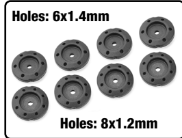
C-00180-768 Shock Piston Heavy Duty - 4mm thick - 1 Set
